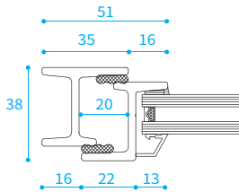
CROSS SECTION 1.3
