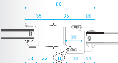
CROSS SECTION 1.7
