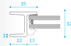
CROSS SECTION 1.1
