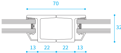
CROSS SECTION 1.5
