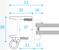
CROSS SECTION 1.4
