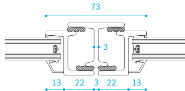
CROSS SECTION 1.8
