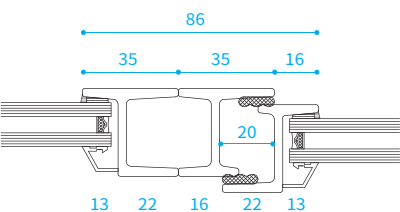
CROSS SECTION 1.6
