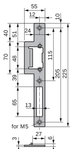
Illustration: active leaf DIN right
