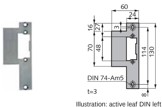
Illustration: active leaf DIN left
