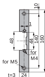
Illustration: active leaf DIN left
