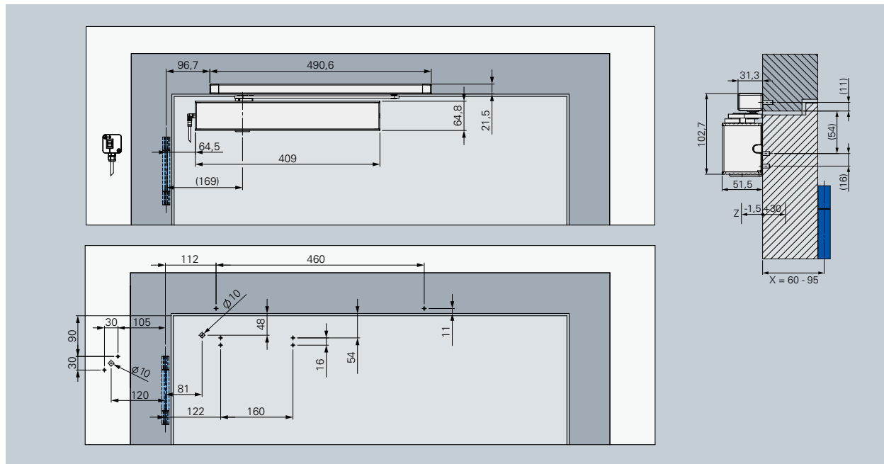
标准安装，铰链背侧，DIN-R - ECO FTS III
