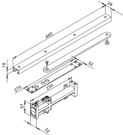
尺寸: ITS 380
