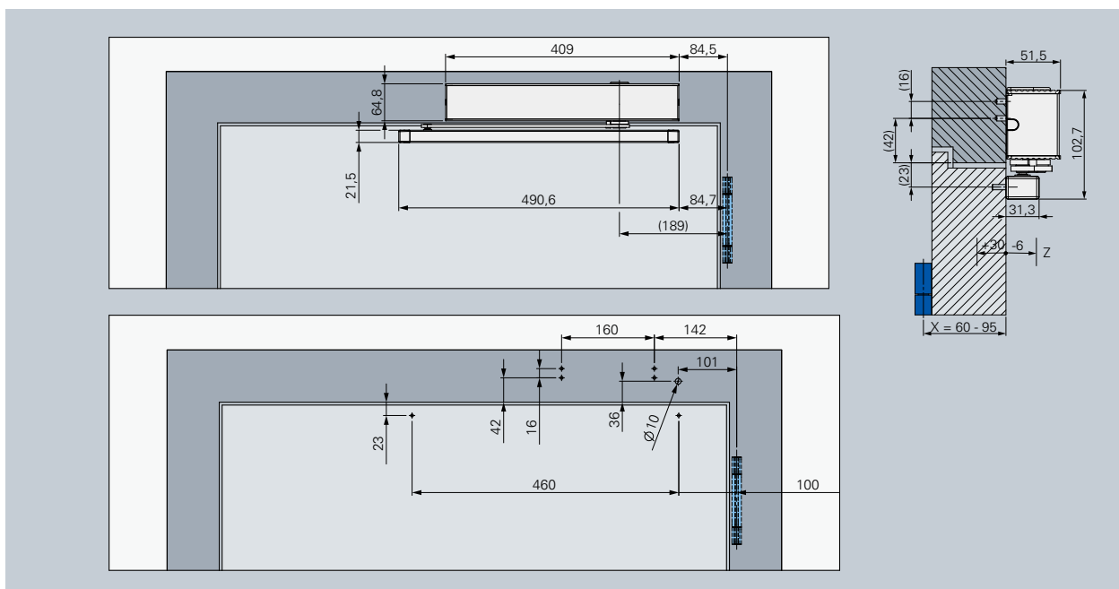
顶部安装，铰链背侧，DIN-R - ECO FTS III
