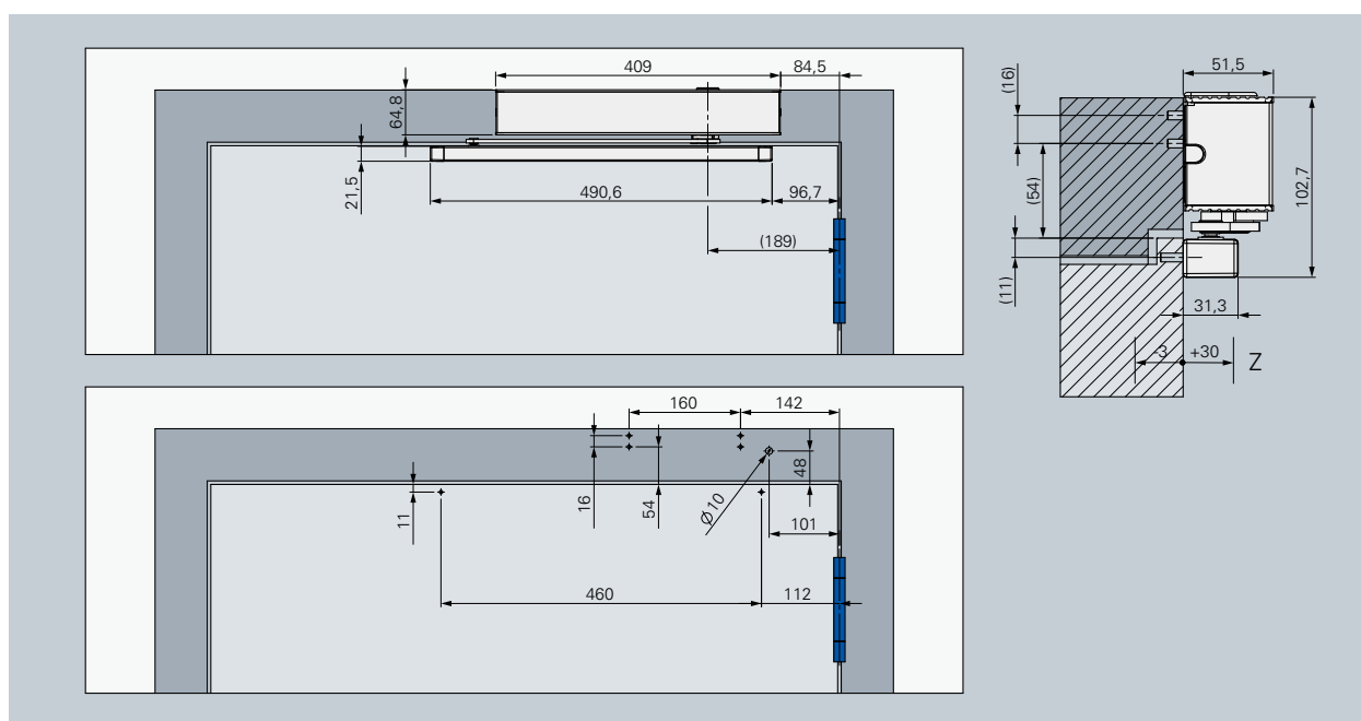
顶部安装，铰链侧，DIN-R - ECO FTS III
