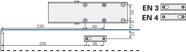
关门力度级别EN 3/4
