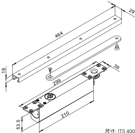
尺寸: ITS 400
