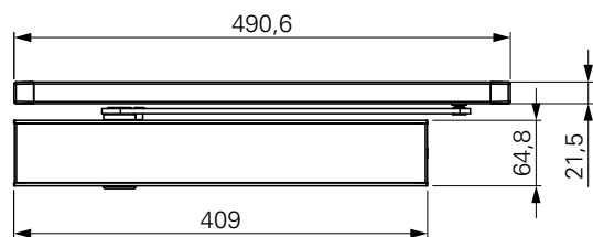
尺寸: ECO FTS III
