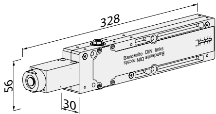
尺寸: ITS Multi-Genius
